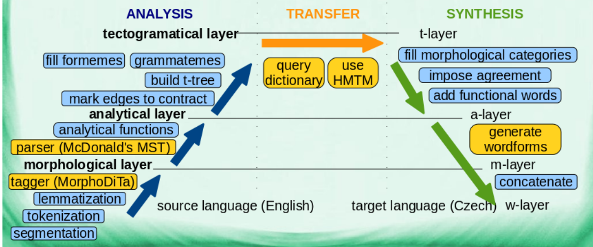
Figure 1: TectoMT architecture (Popel, 2014)
